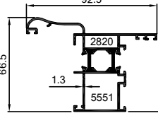
55-2820-5551 1.484 kg/m
