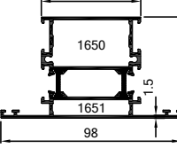
55-5154-5155 2.370 kg/m
