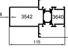
55-3640-3542 2.376 kg/m
